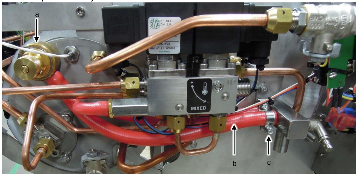
Showing the new version pressure safety valve.
